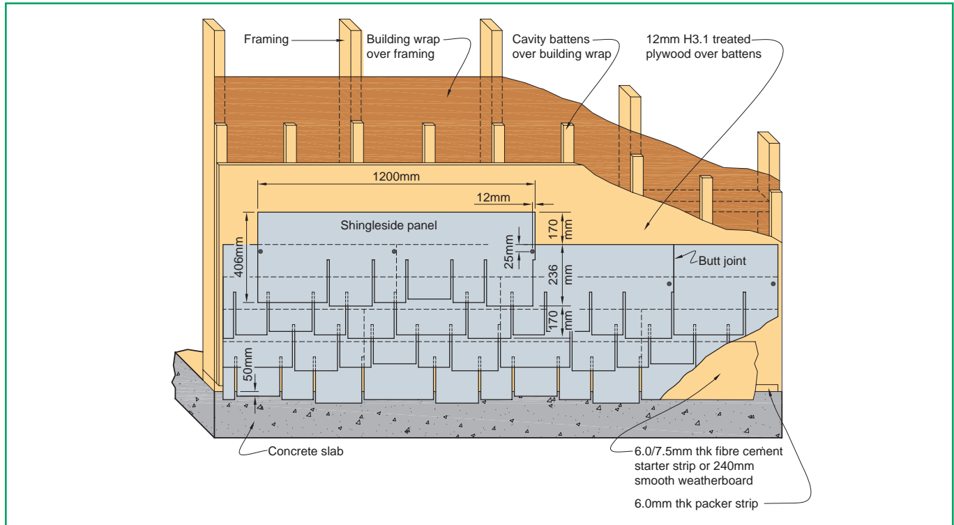
FIGURE 1: SHINGLESIDE PANEL (STAGGERED EDGE)
