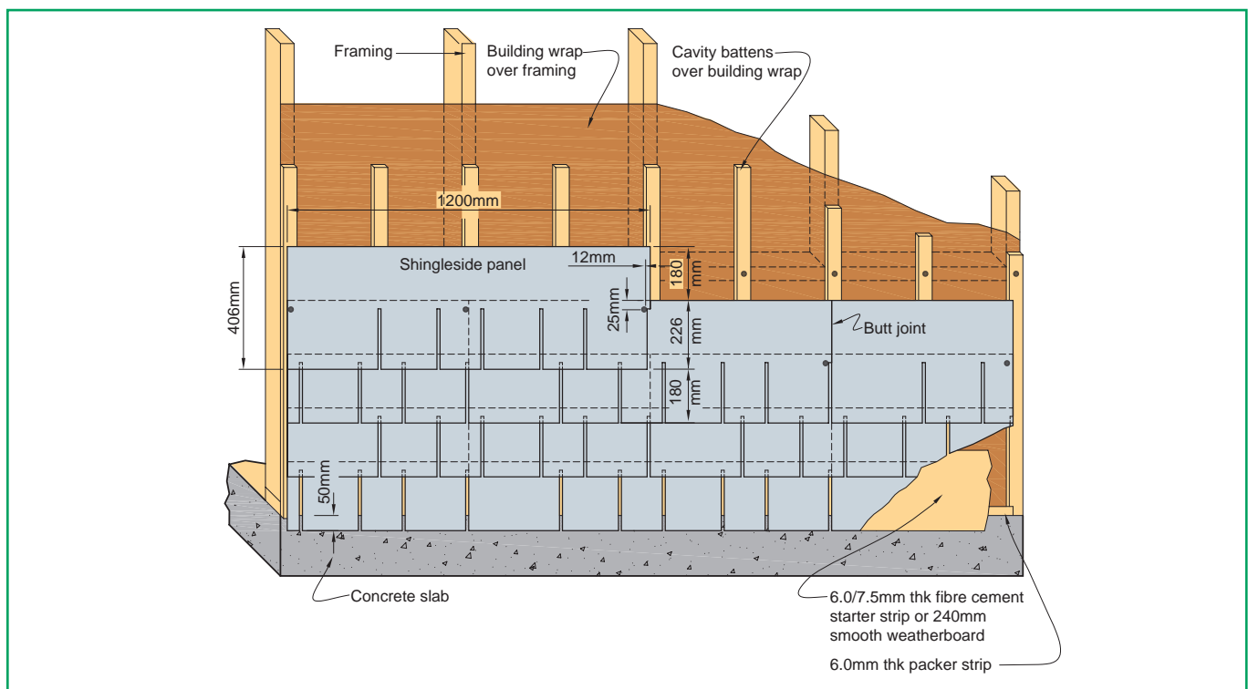
FIGURE 2: SHINGLESIDE PANEL (STRAIGHT EDGE)
