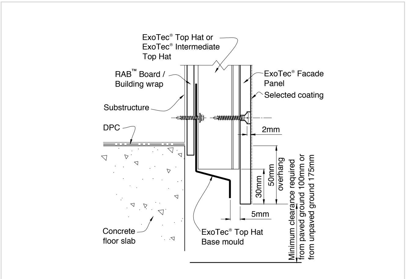
Figure 4: Wall base typical detail
