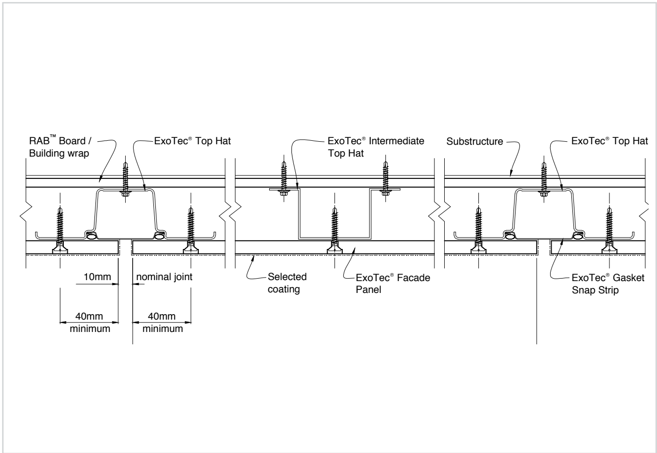
Figure 5: Top Hat and panel fixing detail
