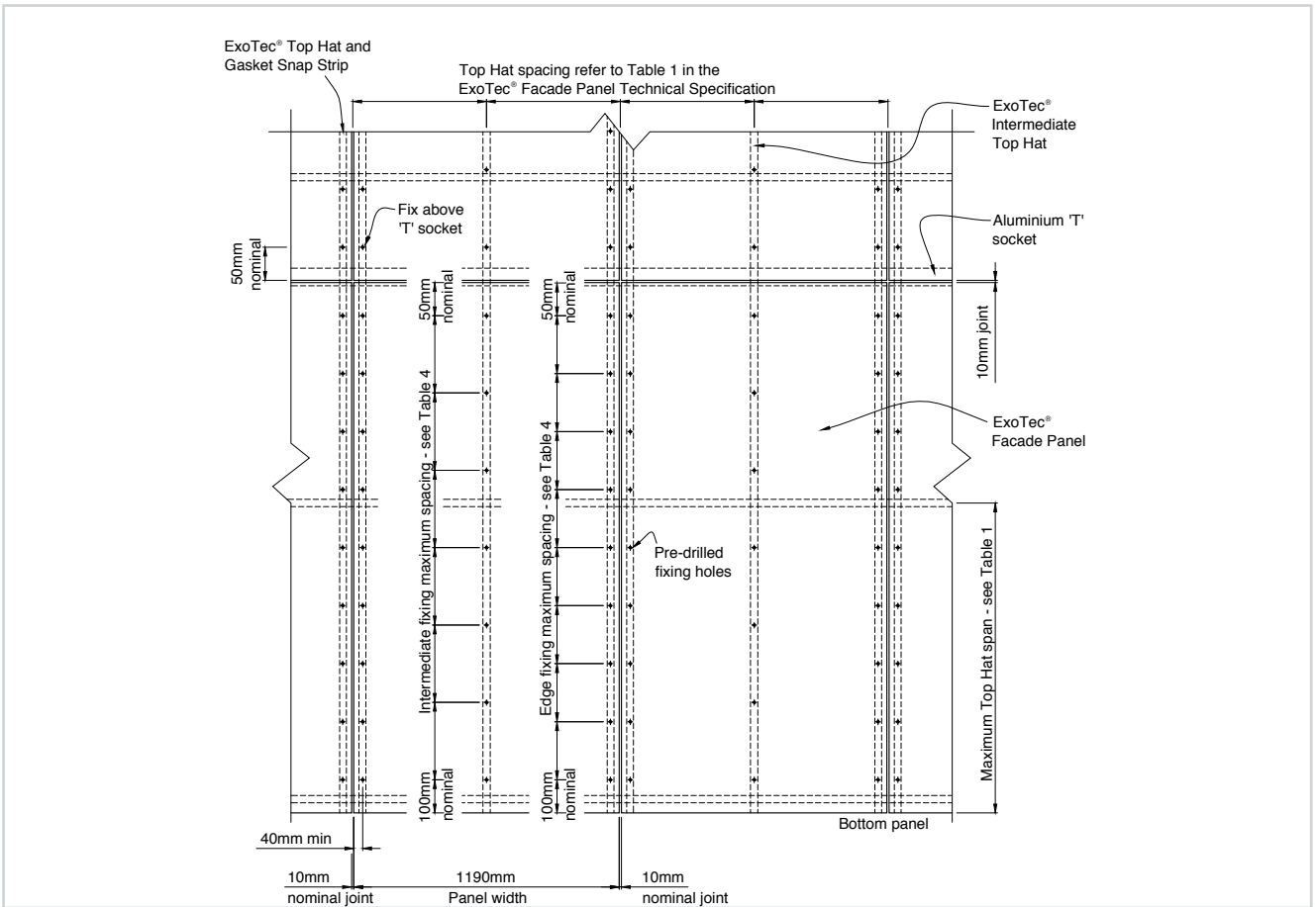
Figure 3: Typical panel and framing layout
