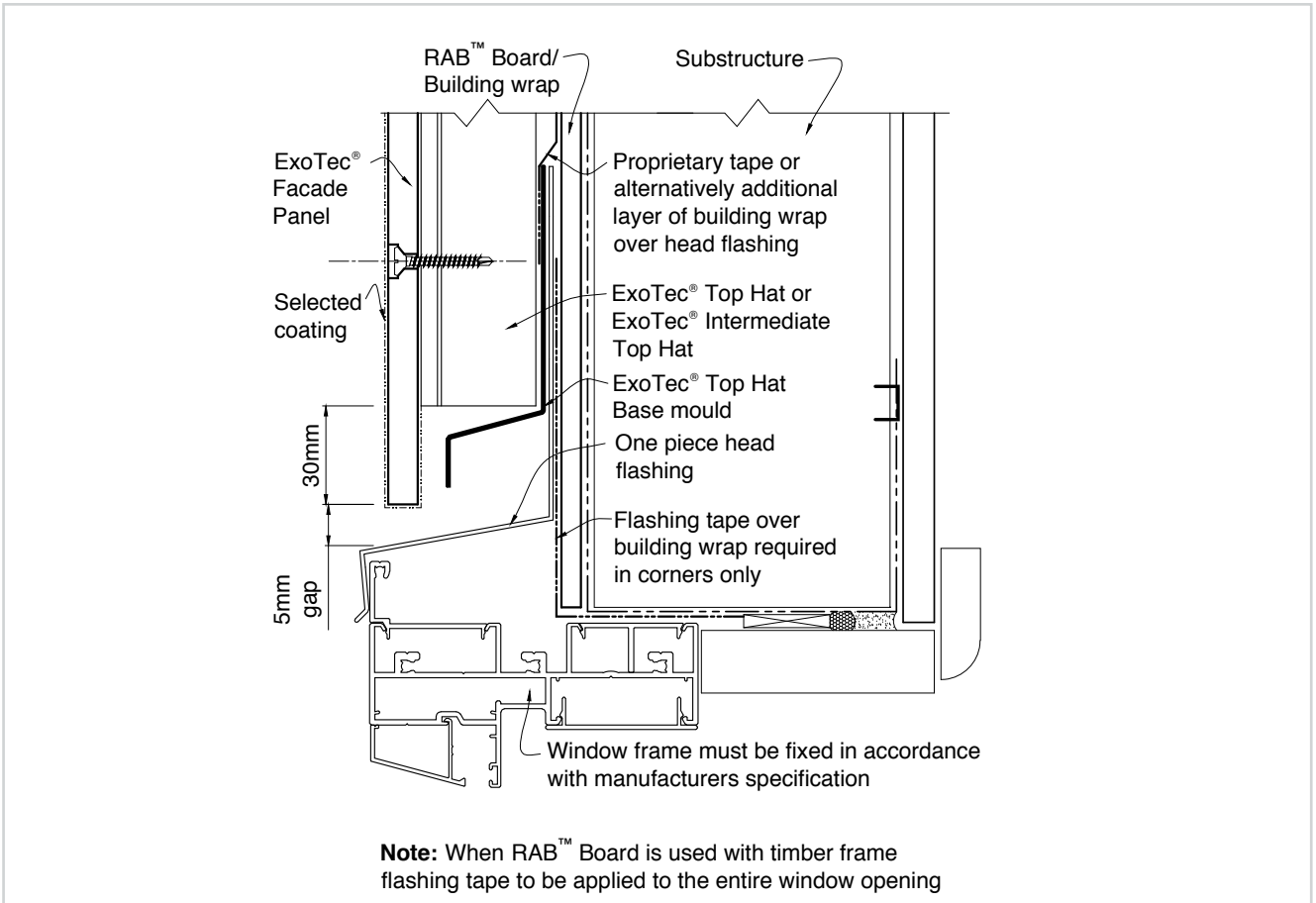
Figure 17: Commercial window head detail
