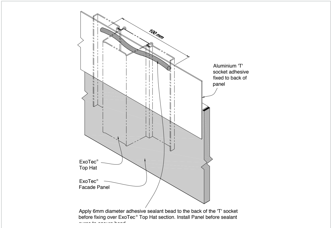
Figure 23: Sealing aluminium 'T' socket to ExoTec® Top Hat
