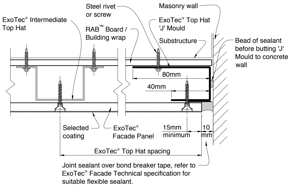
Figure 26: ExoTec Facade Panel and masonry wall abutment
