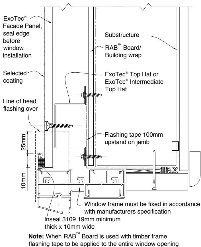
Figure 15: Commercial window jamb detail
