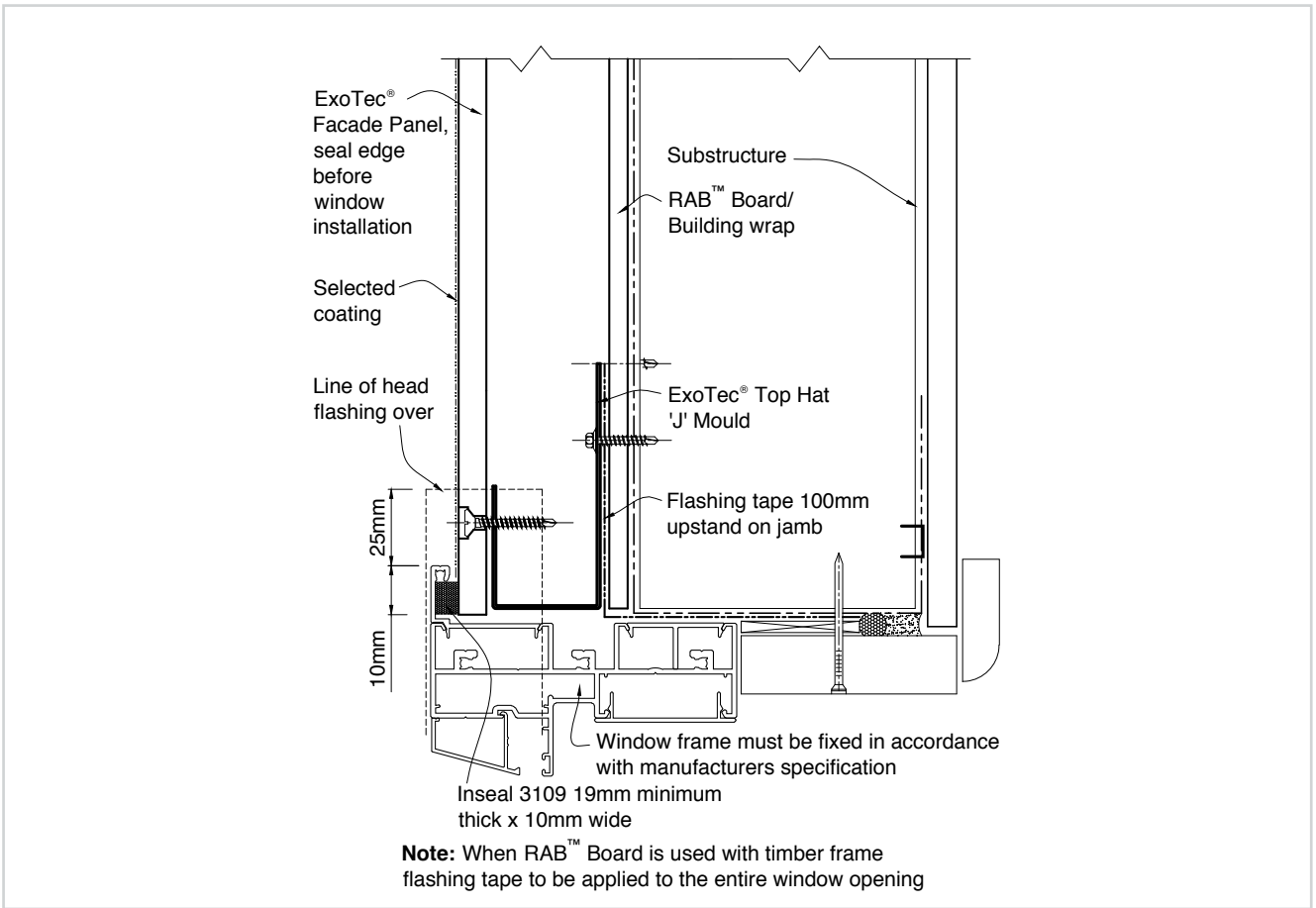
Figure 16: Commercial window jamb detail using 'J' Mould
