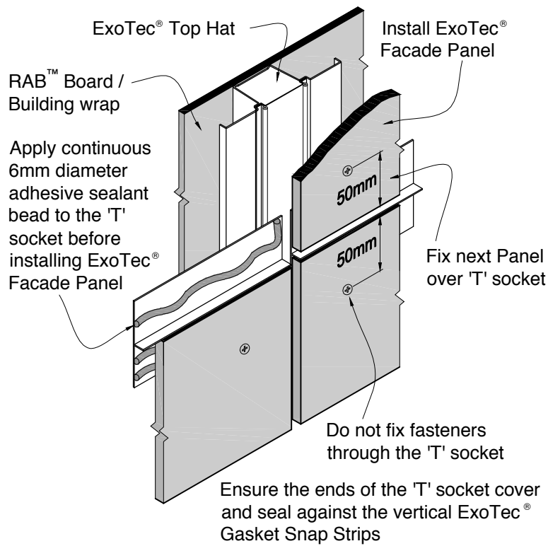
Figure 20: Installing upper panel over aluminium 'T' Socket
