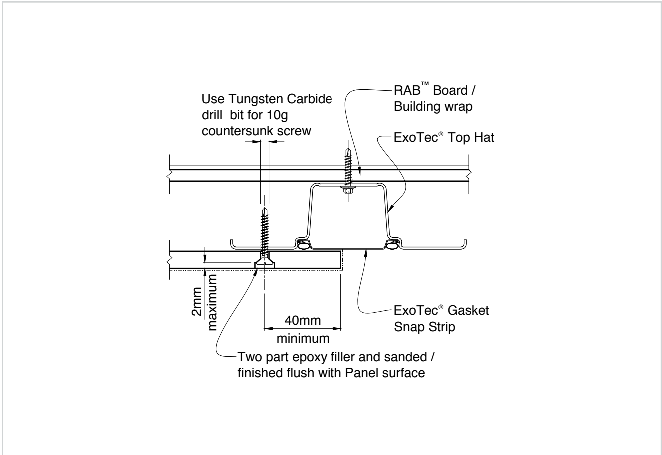
Figure 6: Countersunk fastener detail
