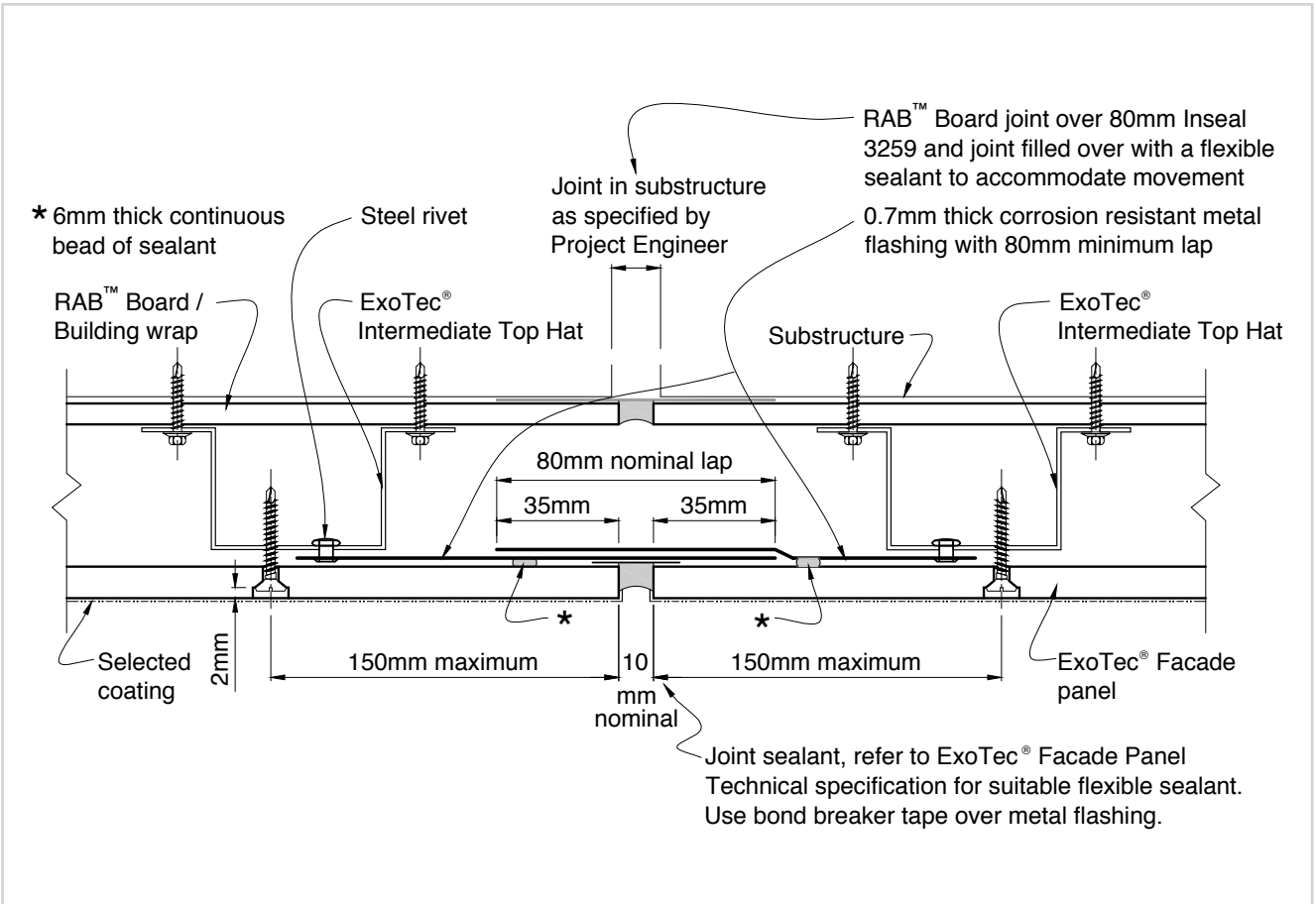
Figure 25: Vertical structural joint detail
