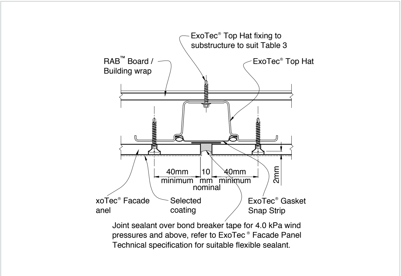
Figure 8: Panel joints in high wind pressure areas detail
