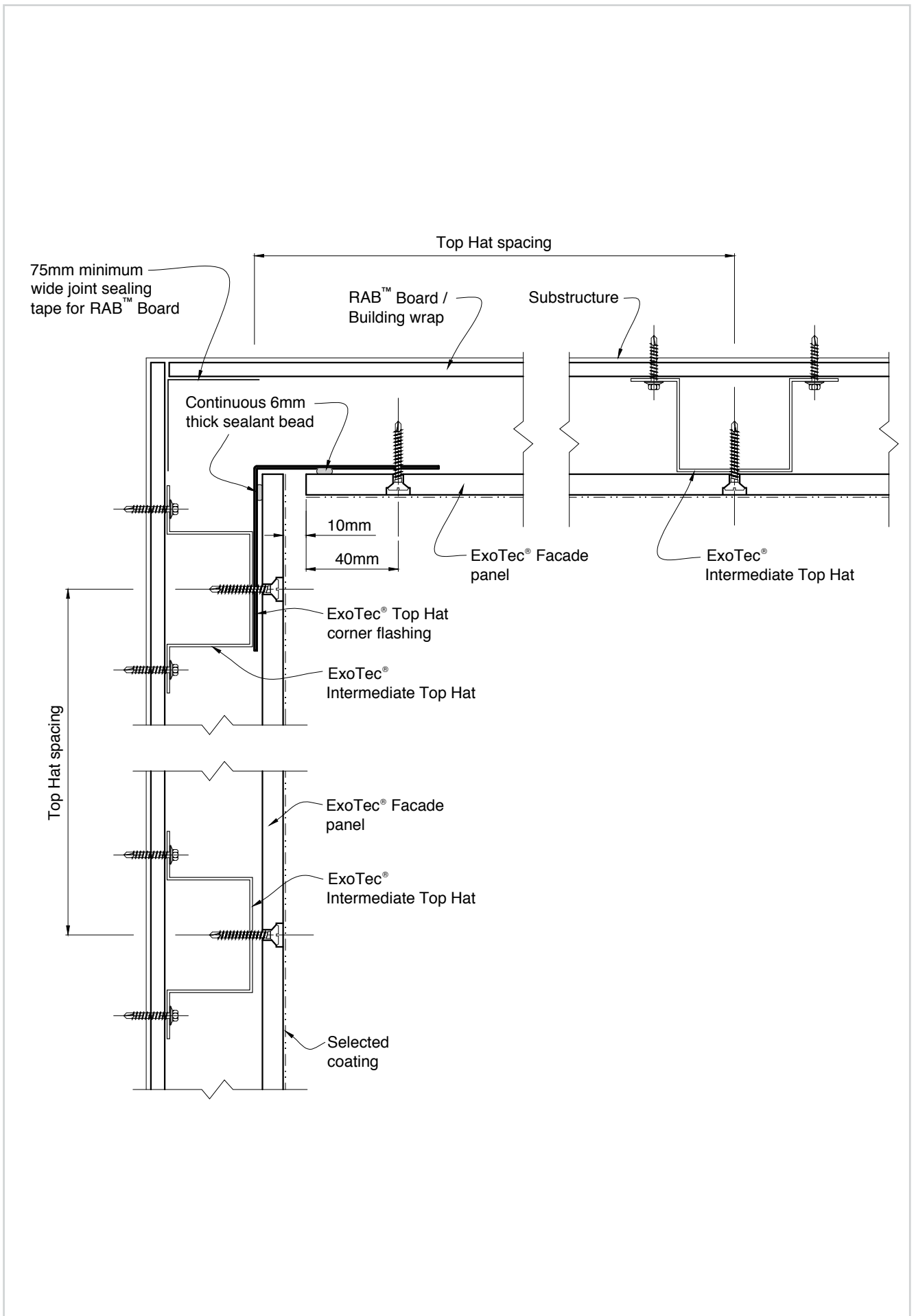
Figure 11: Internal corner detail
