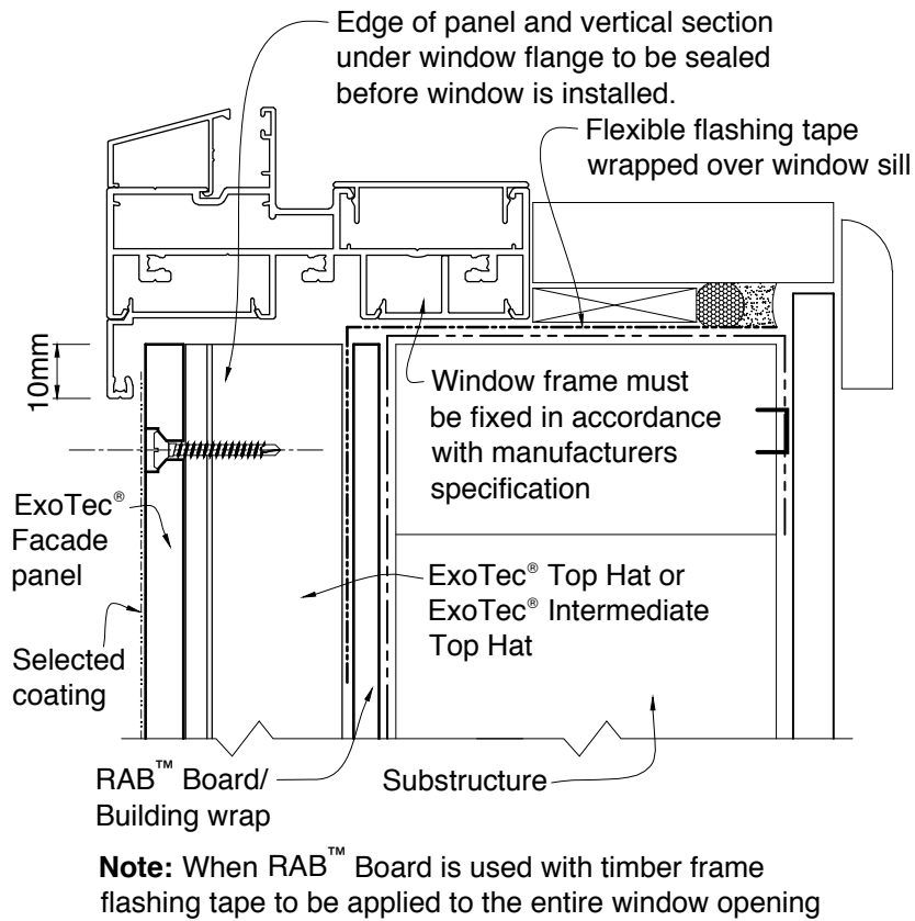
Figure 14: Commercial window sill detail
