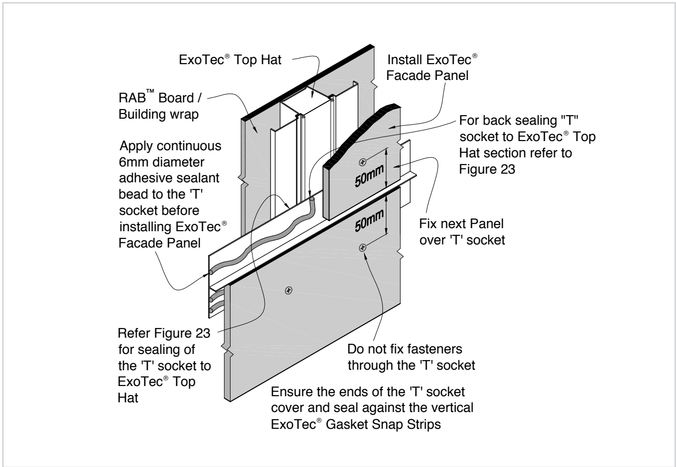
Figure 22: Vertical joint terminating over the horizontal joint
