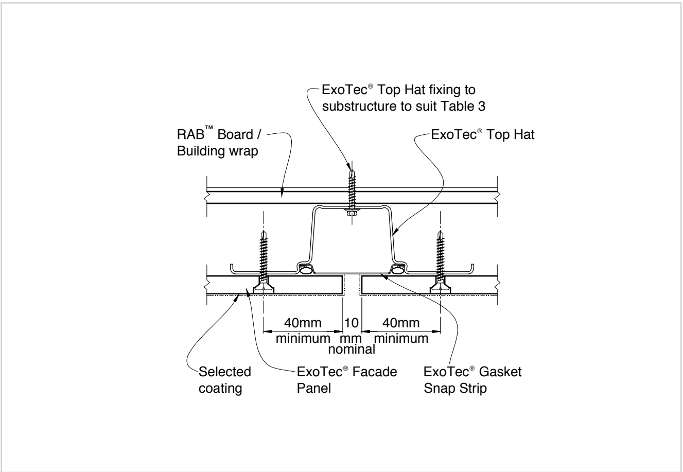
Figure 7: Vertical panel joint detail
