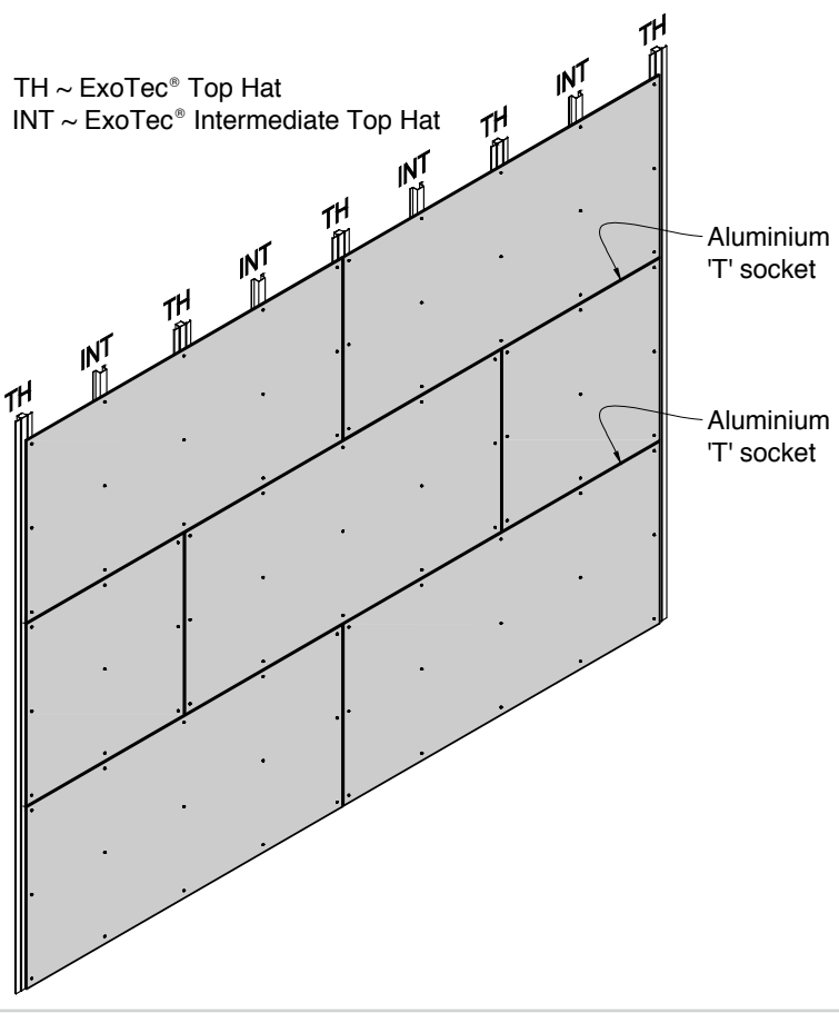
Figure 1: Horizontal layout brick grid pattern
