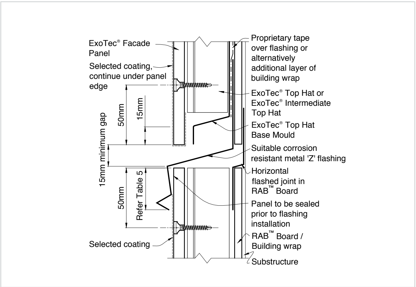
Figure 24: Horizontal structural joint detail
