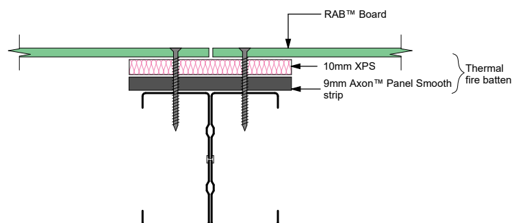
Figure 1: Thermal Fire Batten Fixing
