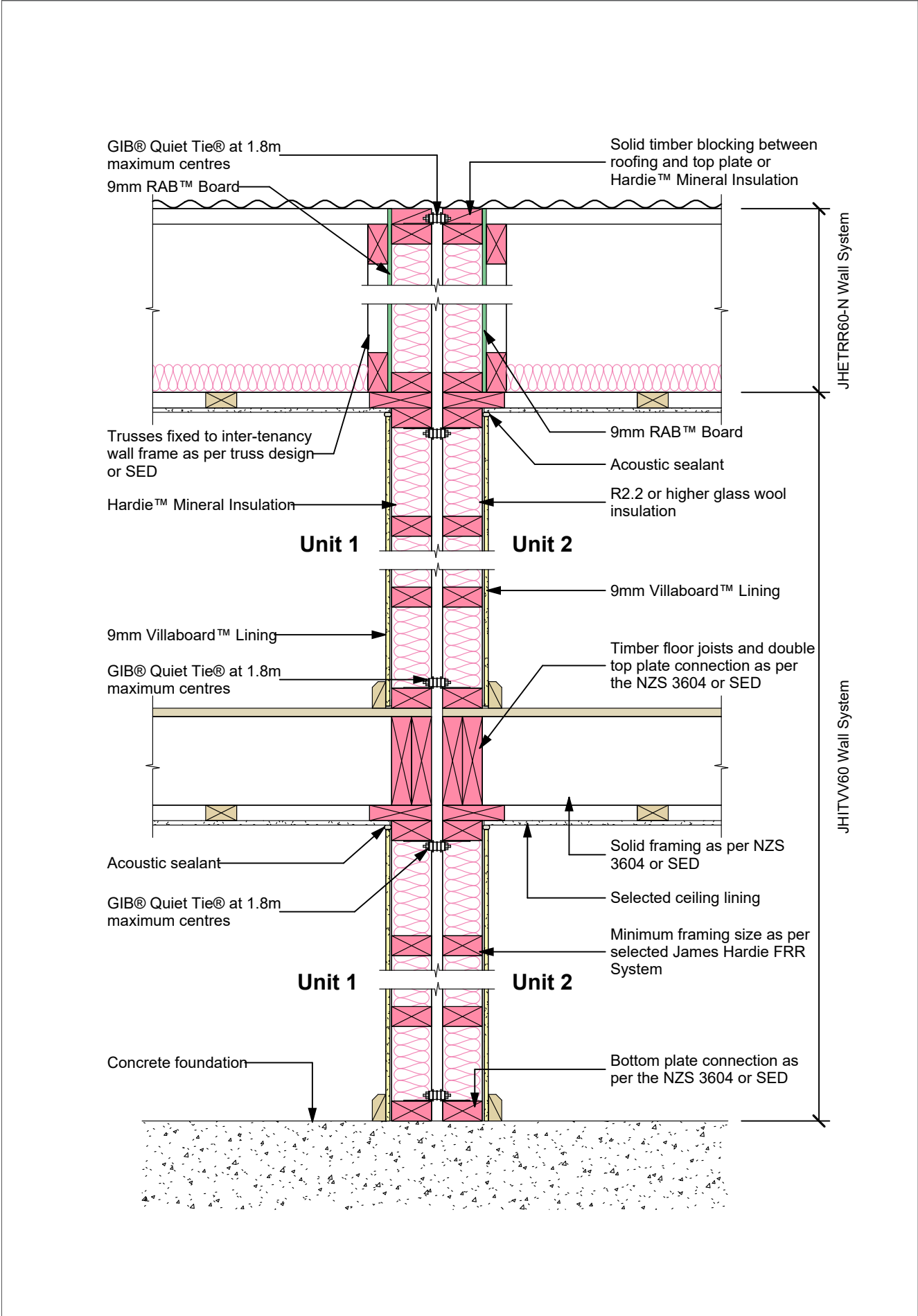
Figure 12: Intertenancy Wall Multi-Story Detail on Concrete Foundation
