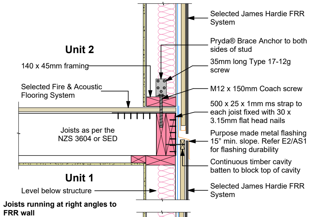
Joists running at right angles to FRR wall
