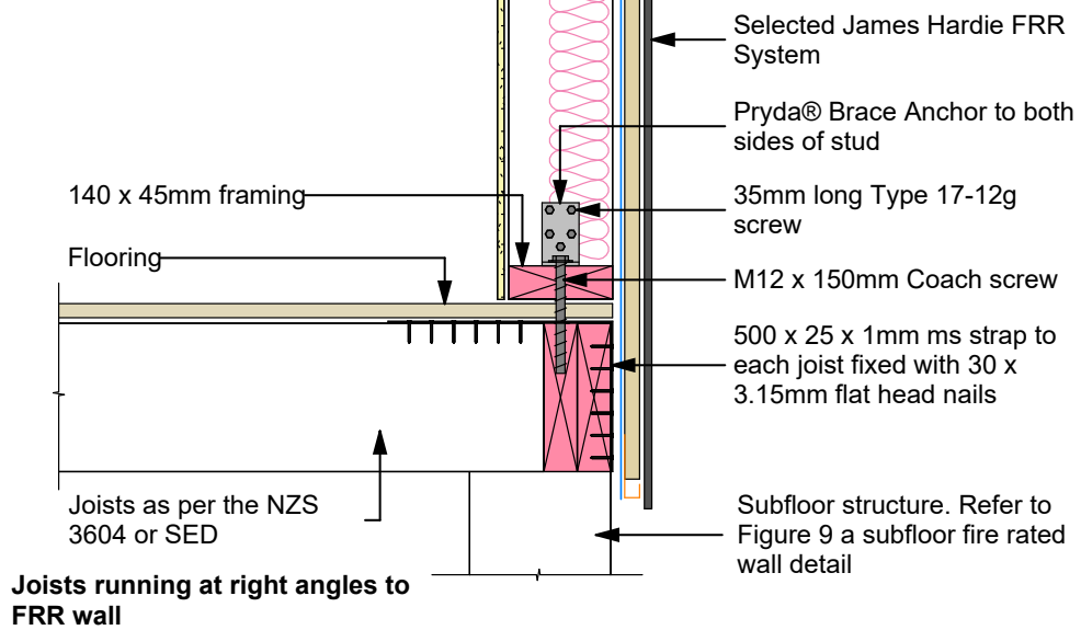
Joists running at right angles to FRR wall
