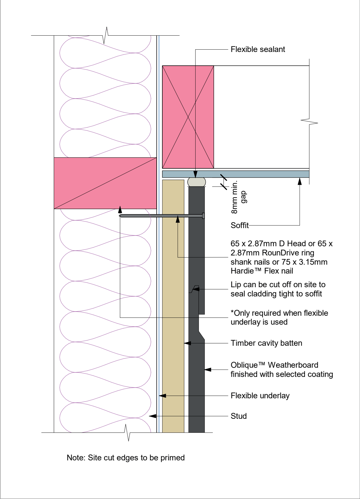
Figure 14: Soffit detail
