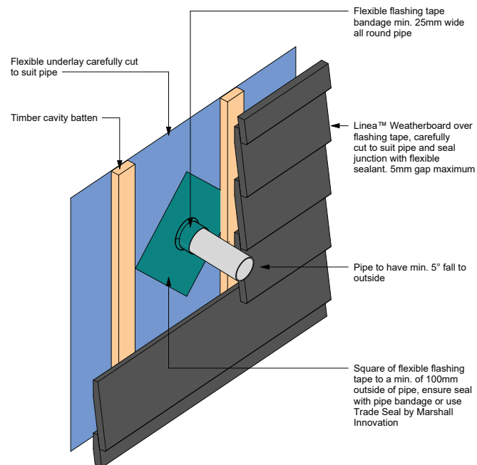
Figure 25: Pipe penetration
