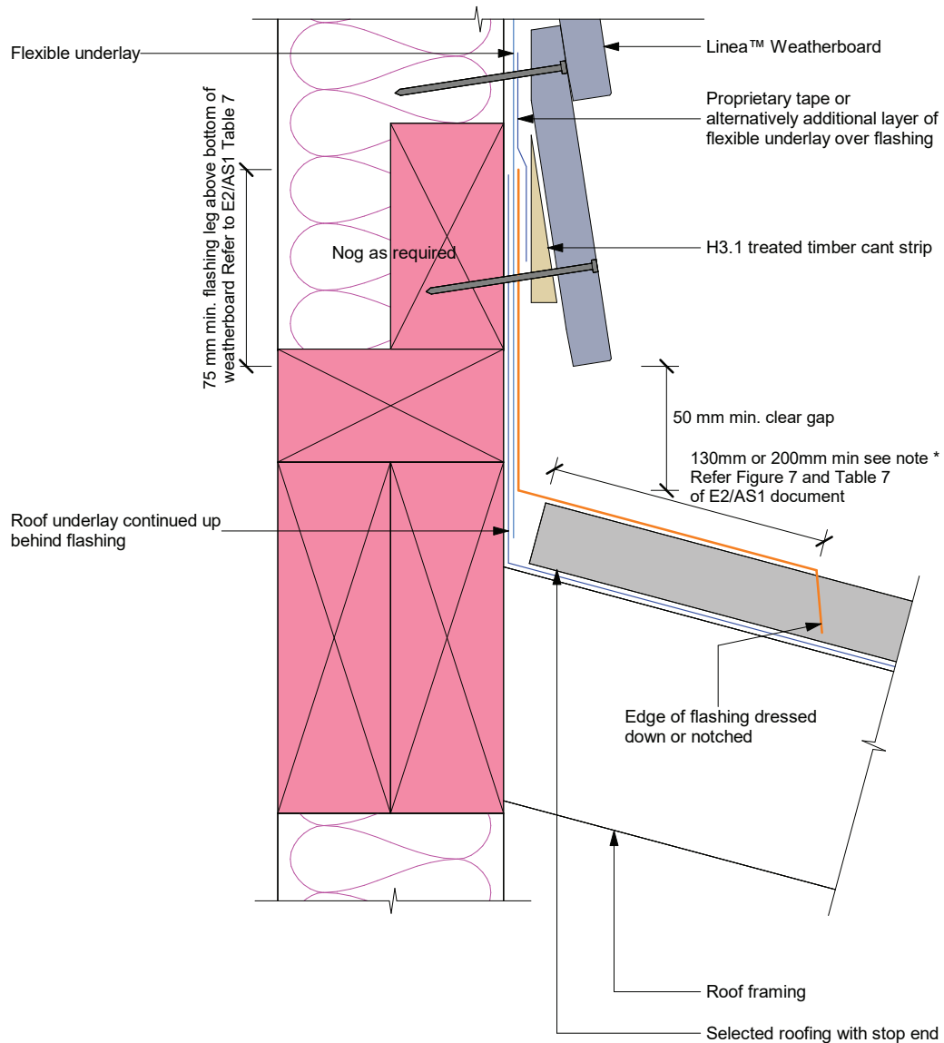
Figure 23: Apron flashing detail
