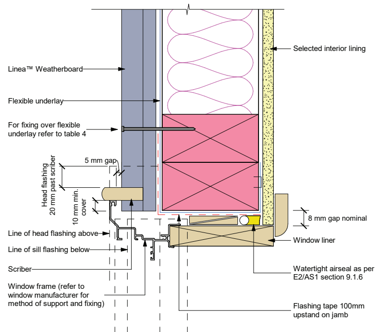
Figure 15: Window jamb
