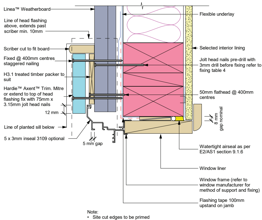
Figure 19: Window jamb with facing
