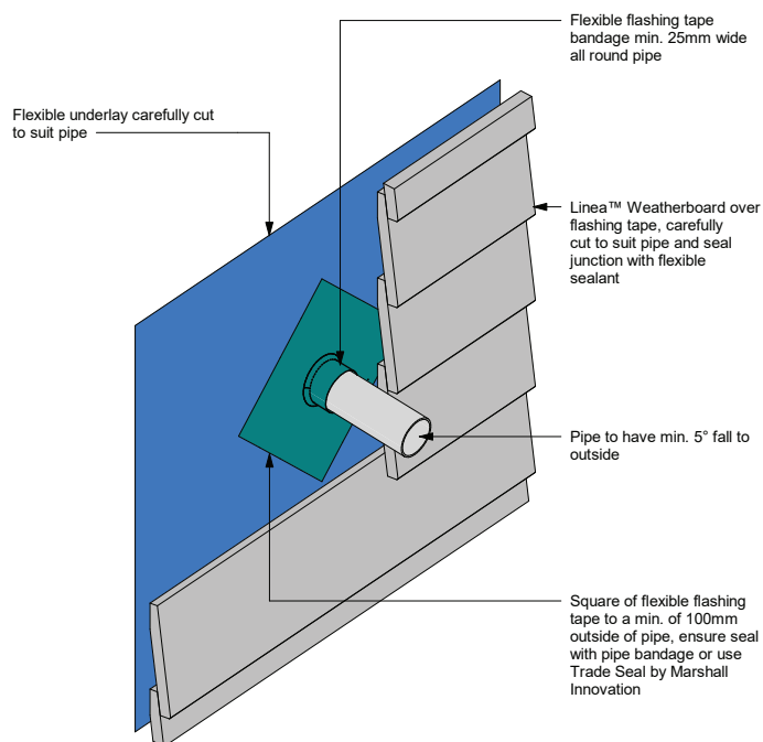
Figure 20: Pipe penetration
