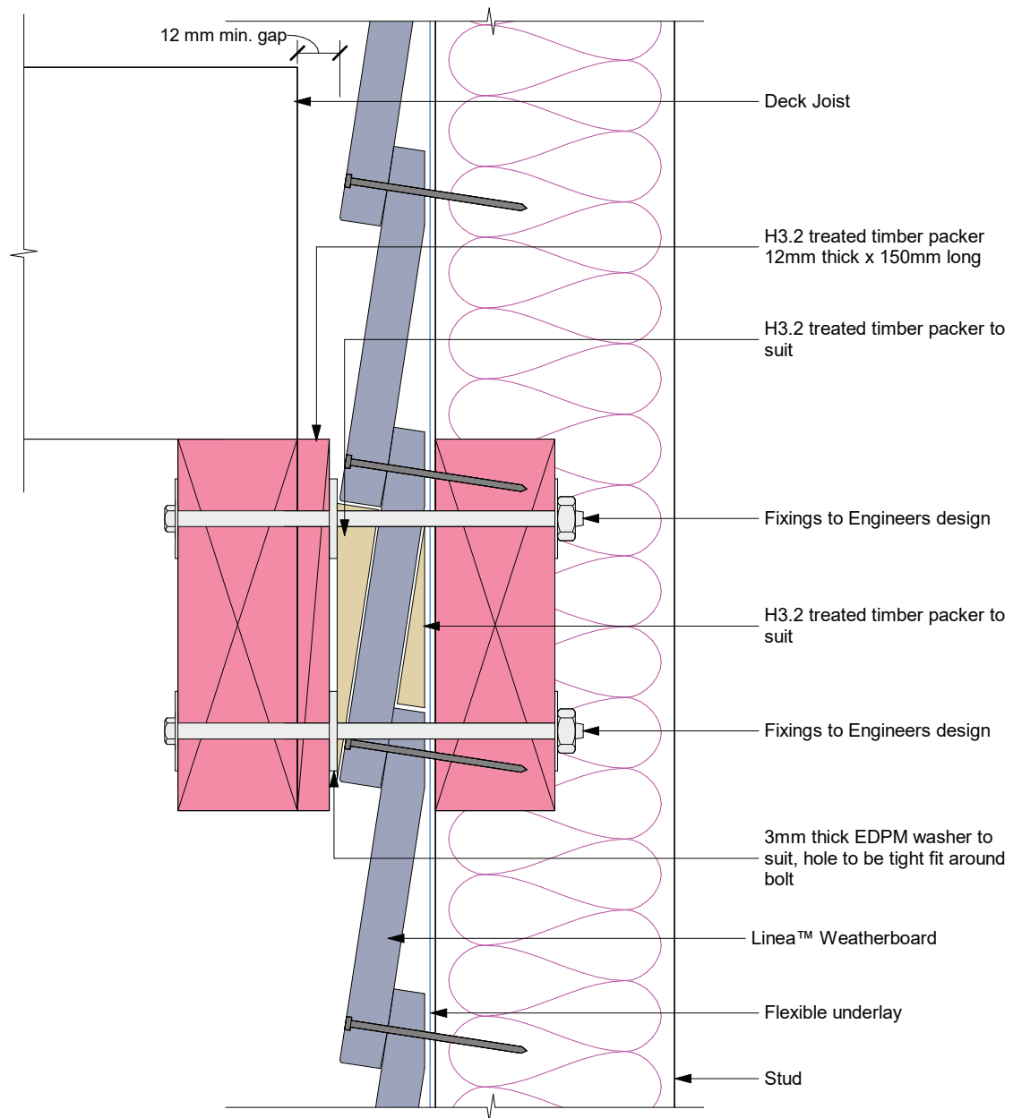
Figure 22: Timber deck junction
