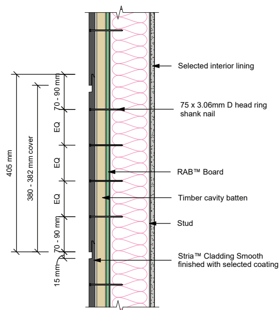
Figure 10: 405mm - Cladding fixing above EH Wind Zone to 3.2kPa wind pressure
