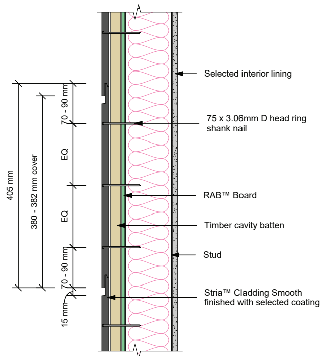
Figure 8: 405mm - Cladding fixing up to EH Wind Zone
