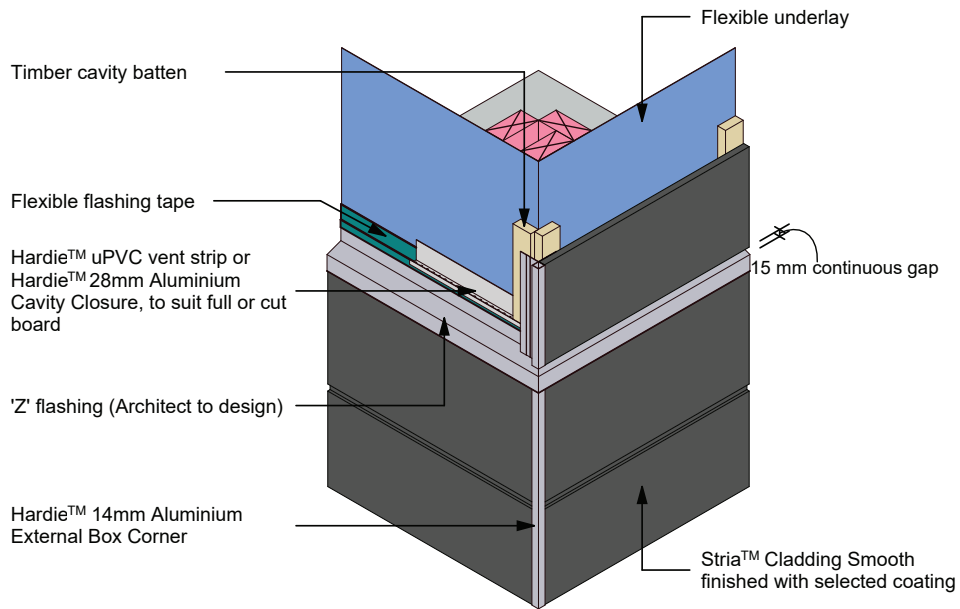
Figure 37: Drained flashing joint at external corner
