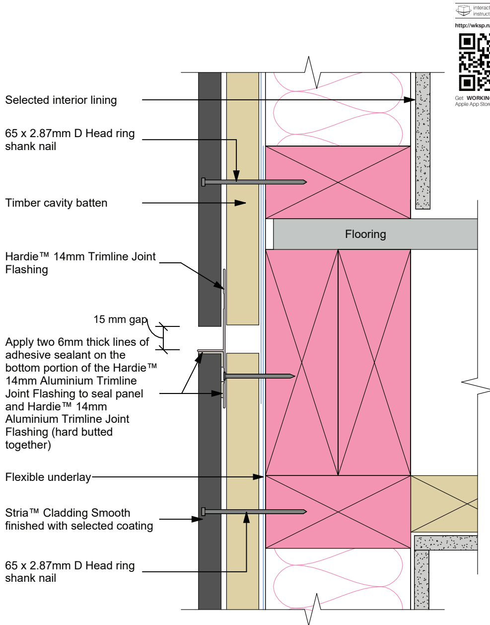
Figure 29: Trimline Horizontal joint at floor joist level
