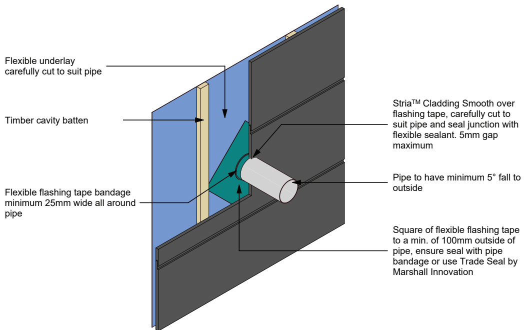
Figure 38: Pipe penetration
