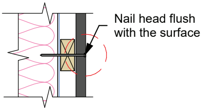
RoundDrive Nail (Plan view)
