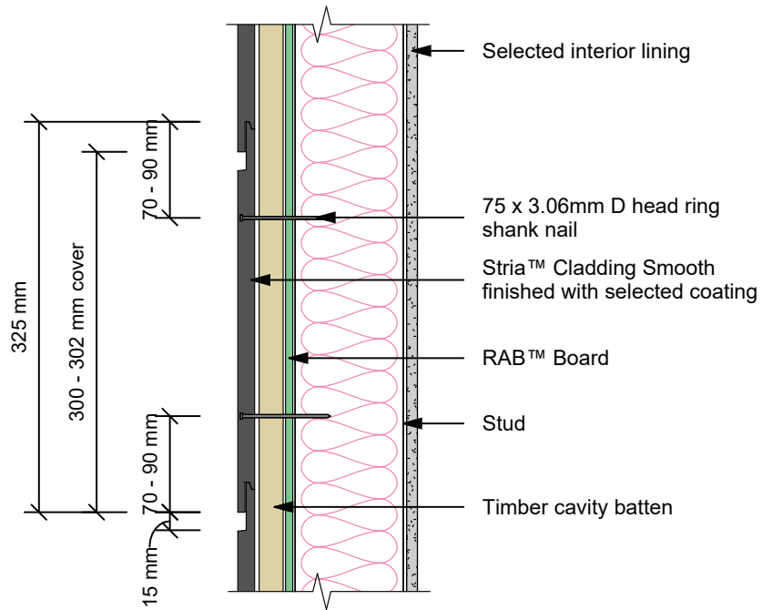
Figure 7: 325mm - Cladding fixing up to EH Wind Zone
