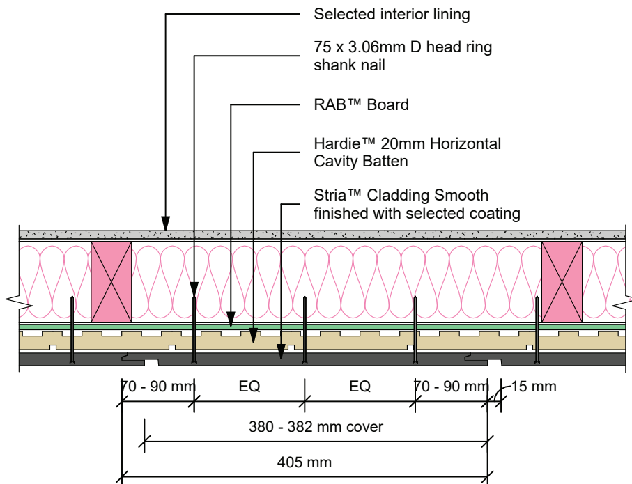
Figure 7: 405mm - Cladding fixing up to EH Wind Zone
