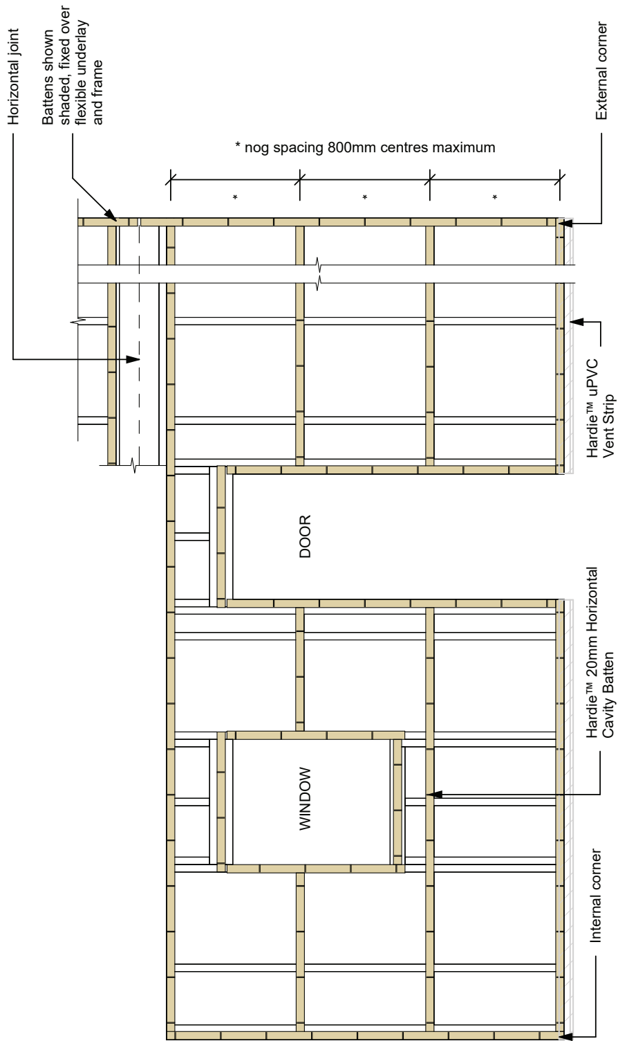
Figure 1: Framing set out
