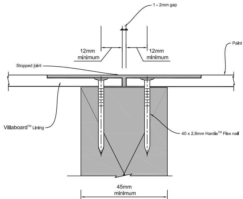
Figure 13: Vertical flush joint setout
