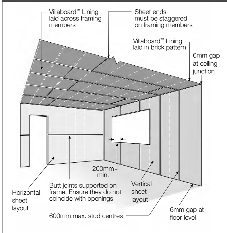
Figure 2: Sheet layout
