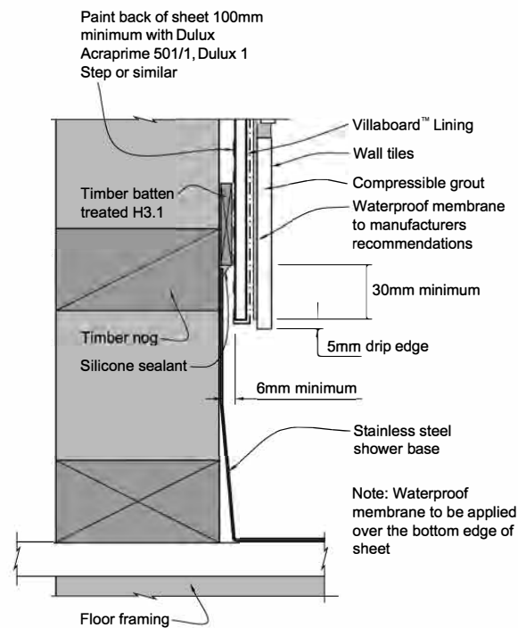
Figure 25: Wall to stainless steel shower
