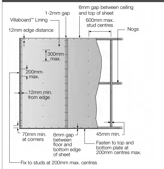
Figure 7: Fastening to wall frames
