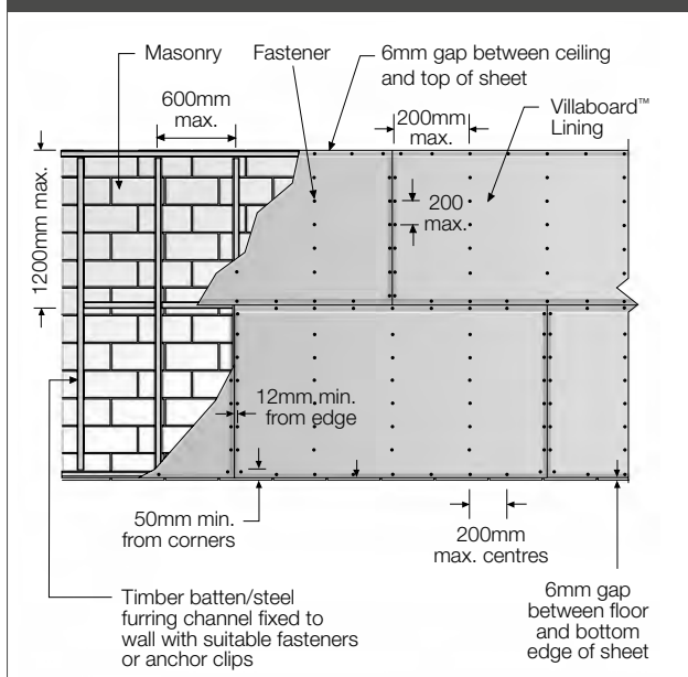
Figure 12: Batten/furring channel – horizontal layout
