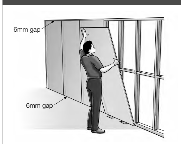
Figure 3: First sheet
