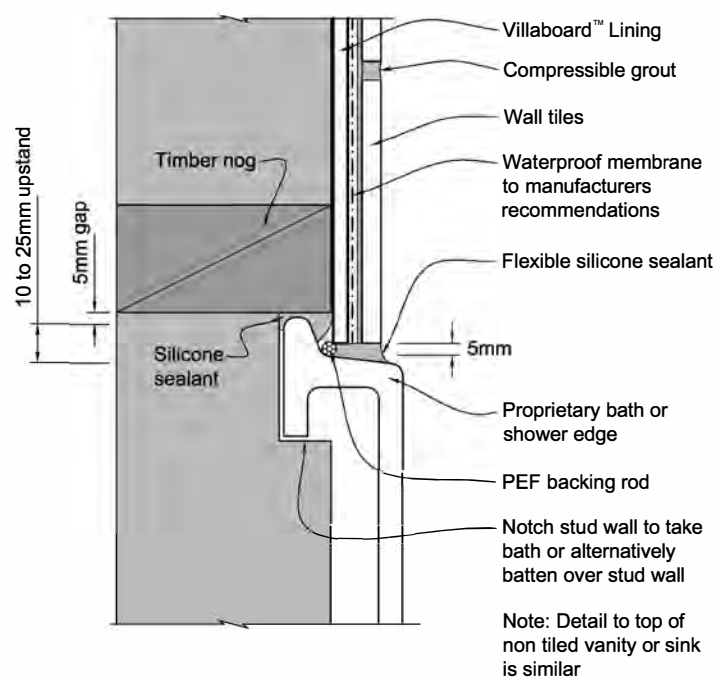
Figure 24: Wall to acrylic bath/shower
