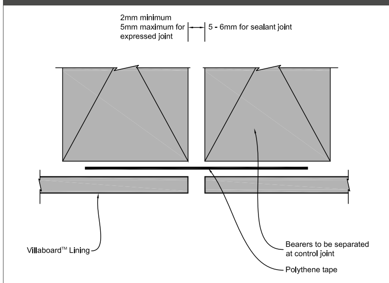
Figure 19: Control joint
