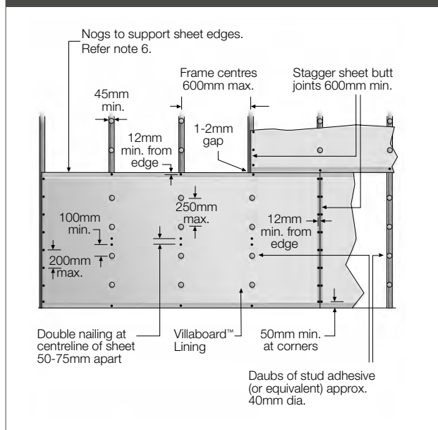
Figure 11: Fastener/adhesive fixing to ceiling
