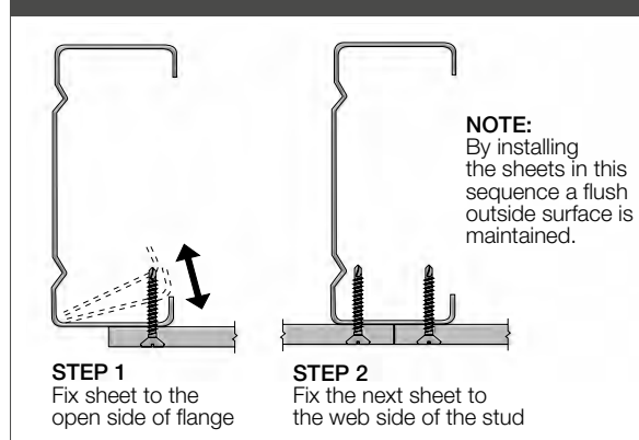
Figure 6: Screw fastening
