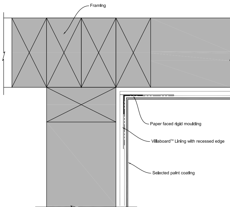
Figure 14: Wall to wall junction
