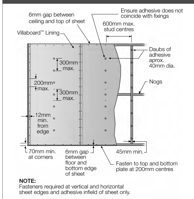
Figure 8: Fastener/adhesive fixing to wall frames
