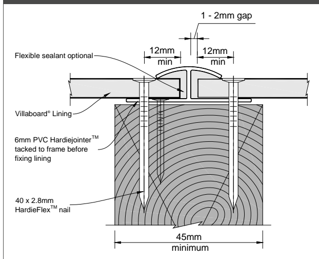
Figure 17: Butt joint detail
