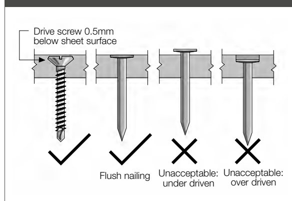
Figure 5: Fastener depth
